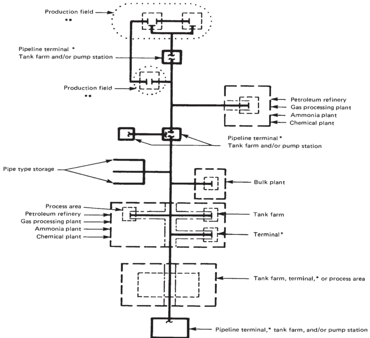
Fig. 400.1.1-1 Diagram Showing Scope of ASME B31.4 Excluding Carbon Dioxide Pipeline Systems (See Fig. 400.1.1-2)
